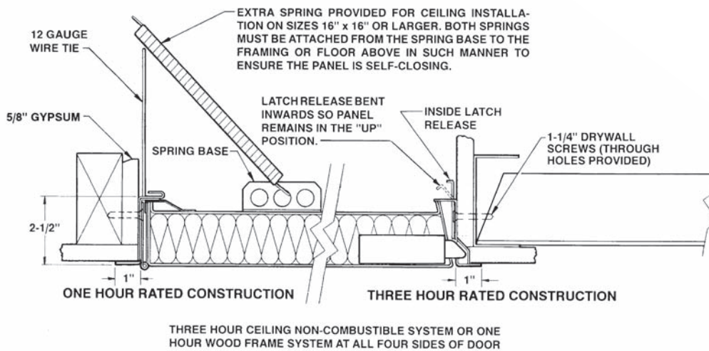
ADFR Fire Rated Door
