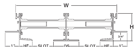
Type HF (2-Slot) Tape & Mud
