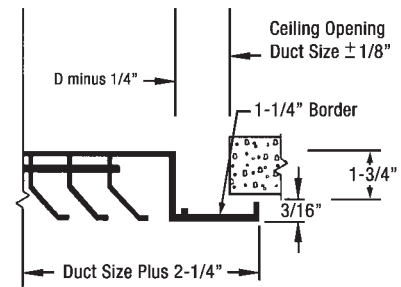
AM5 (Surface Mount, Flat Frame)
