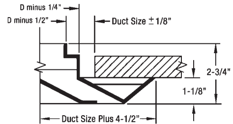
AM6 (Surface Mount, Beveled Frame)
