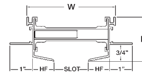
Type HF (1-Slot) Tape & Mud
