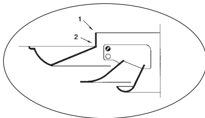
AR2 2-Position Adjustment
