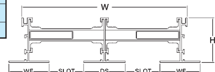
Type WF (2-Slot) Exposed flange
