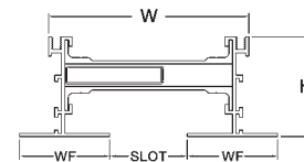
Type WF (1-Slot) Exposed flange
